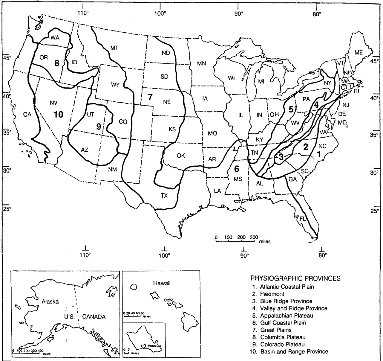
U.S. Physiographic Map
