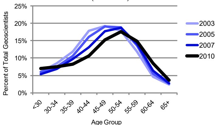
Age Distribution of Geoscientists in the U.S. Government (2003-2010)
