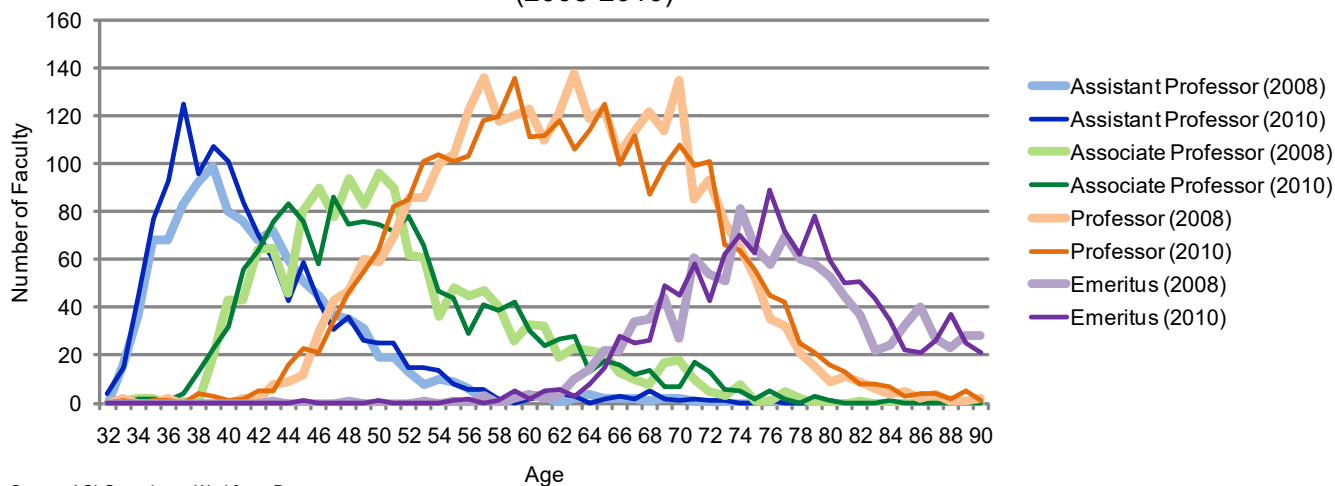
Number of Geoscience Faculty by Age and Rank (2008-2010)
