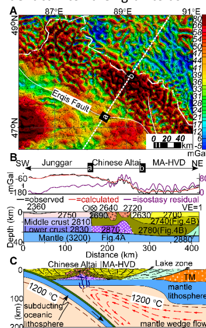
Figure 1: Tectonic interpretation for the generation of the bulk Silurian-Devonian granitoids in the Chinese Altai, in the frame of a gravity model.
