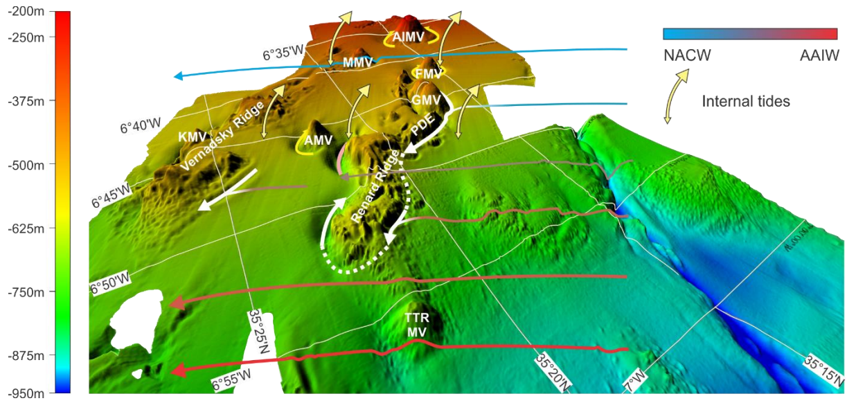
Figure 1: Summarizing figure of all topographies and bottom currents in the El Arraiche area [2].
